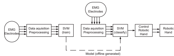
Fig. 1 Data flow plan of the rehabilitation system which consists mainly of EMG data acquisition, the support vector machine (SVM) and the robotic hand.
