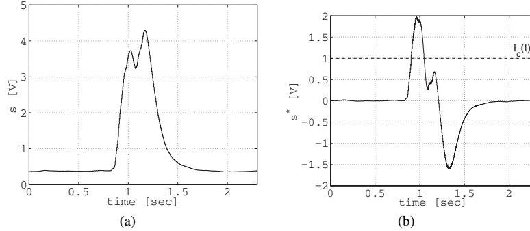
Fig. 3 Muscle activation recorded by one EMG electrode (a) and the same signal high pass filtered (b).
